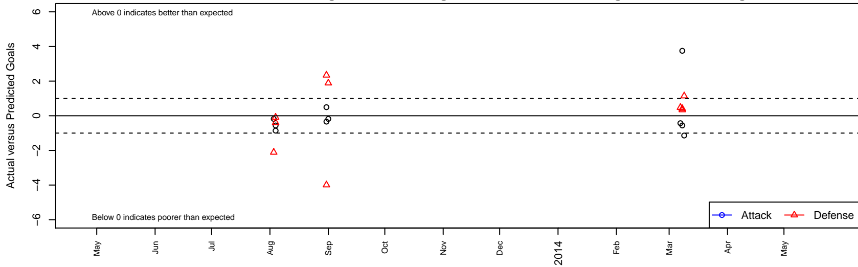
Heat FC 03 MB G02 Dots are actual minus expected GF (blue circles) and GA (red triangles). Blue line is smoothed change in attack strength. Red is smoothed change in defense strength.
